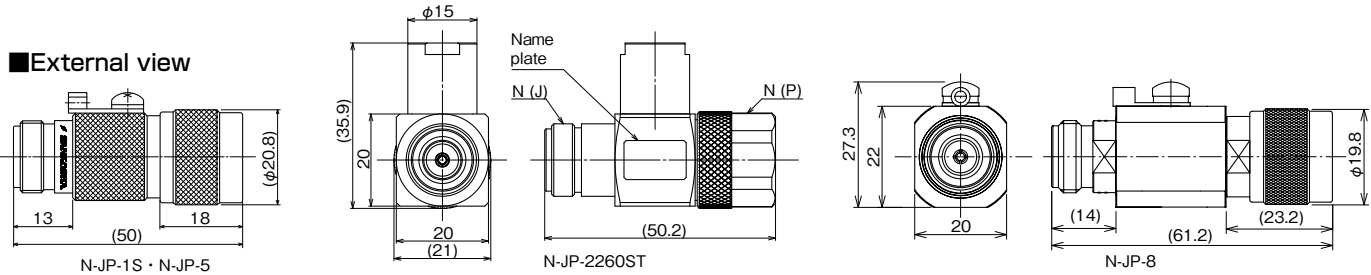
N-JP-1S · N-JP-5 Dimensions: W20.8×D50×H24.3 (mm) Mass: 80 (g)
