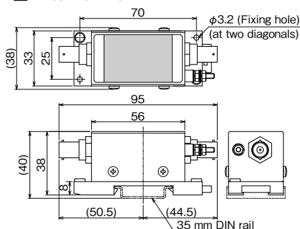
Dimensions: W38×D95×H40 (mm) Mass: 130 (g)
