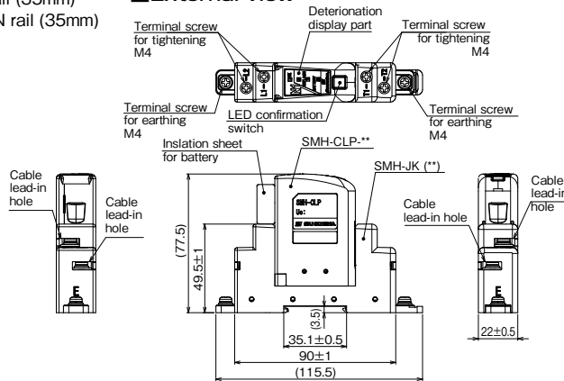
Dimensions: W22×D115.5×H77.5 (mm) Mass: 120 (g)
