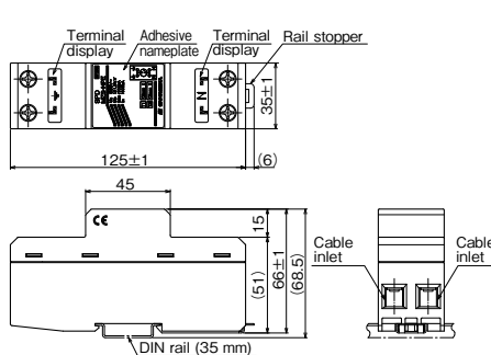
MZS-NPE Dimensions: W35×D125×H66 (mm) Mass: 290 (g)
