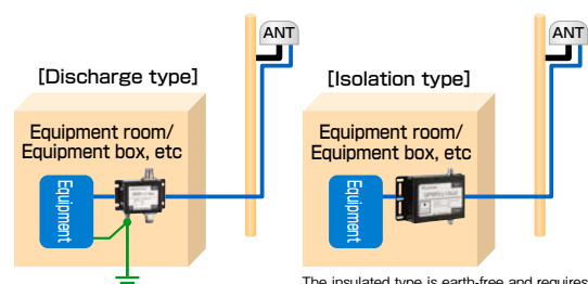
The insulated type is earth-free and requires no grounding work.
